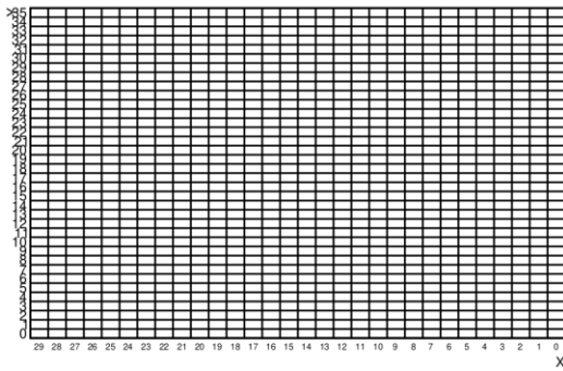
Failed Match Clusters
