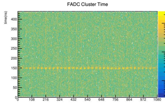
Failed Match Clusters
