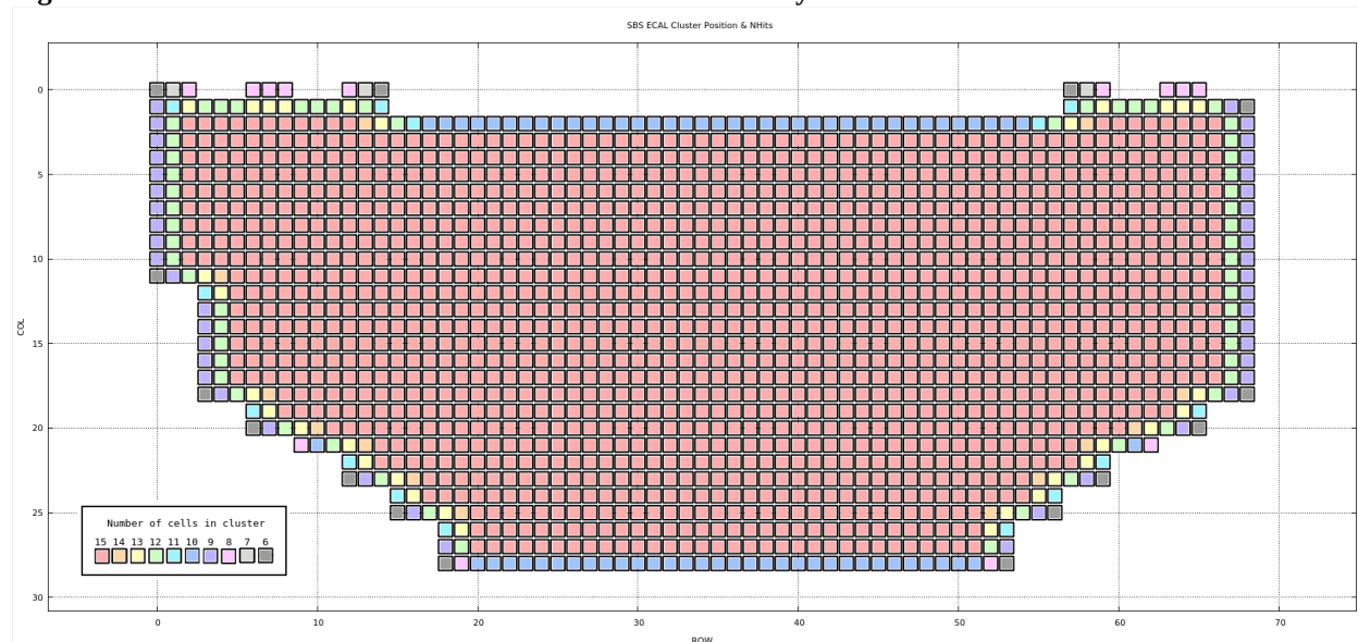
Figure 10.2.2: SBS ECAL cluster scan – calorimeter perimeter cells cluster center removed
